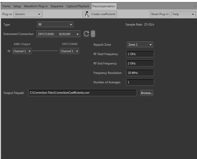
The AWG7000B with the Generic Precompensation plug-in
