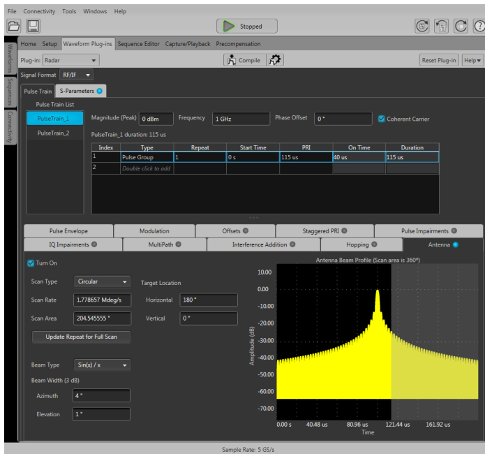
AWG radar pulses created with AWG70000B and Radar plug-in
