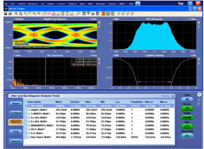
Easily create digital data impairments with the AWG70000B and HSS plug-in
