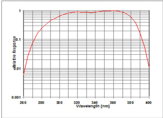
Fig. 1. PMA1107 Spectral Response
